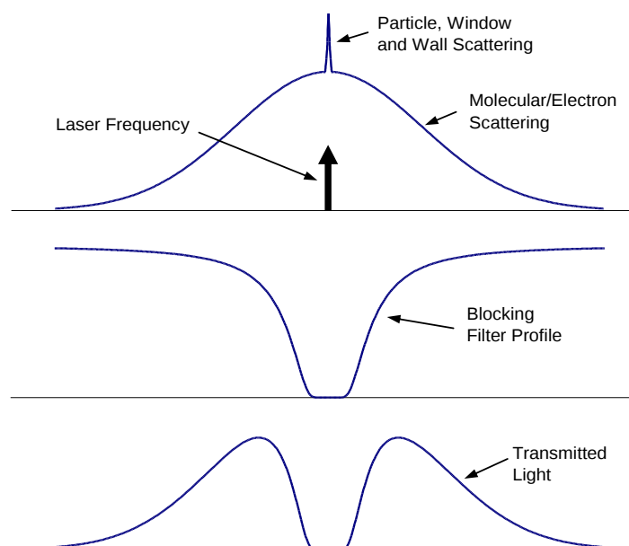
Fig. (4) Basic Filtered Rayleigh Scattering concept
