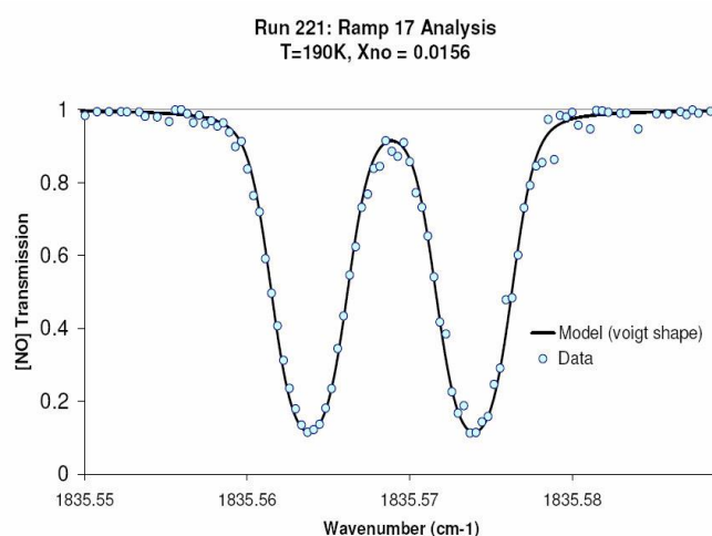
Fig. (2) Single Trace TDLAS spectrum obtained in LENS 1 facility at 5 MJ/kg enthalpy
