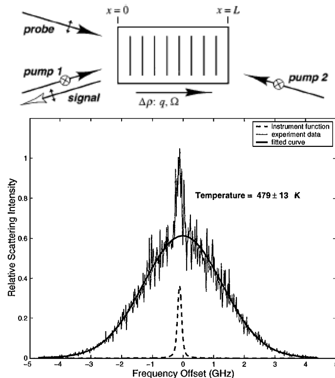
Fig. (7) Schematic illustration of coherent Rayleigh scattering, and example spectrum from argon glow discharge plasma at 50 mbar
