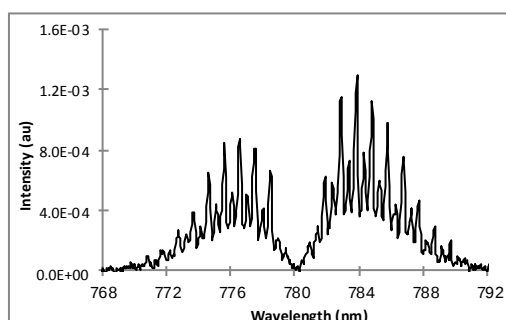
Fig. (5) Pure rotational Raman spectrum of N 2 obtained with a rubidium vapor filter
