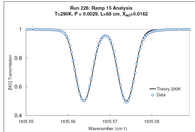
Fig. (3) Single Trace TDLAS spectrum obtained in LENS 1 facility at 10 MJ/kg enthalpy
