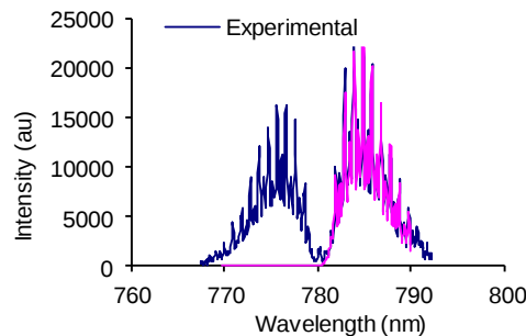
Fig. (6) Filtered pure rotational Raman spectrum of optically pumped \text{N}_2/\text{CO} mixture at 1 bar pressure and least squares spectral fit. Inferred temperature is 355 \pm 7\text{K}
