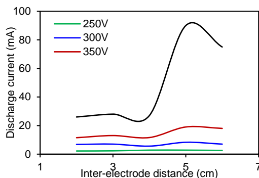
Figure (5) Variation of discharge current with inter-electrode distance at certain discharge voltages without using magnetron
