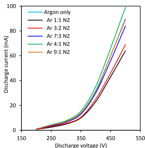
Figure (8) Discharge current-voltage characteristics for different argon/nitrogen mixtures at total gas pressure of 0.7mbar and inter-electrode distance of 4cm
