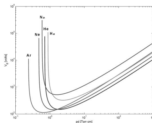
Figure (2) Paschen's curves of different common gases used in electric discharge applications [11]
