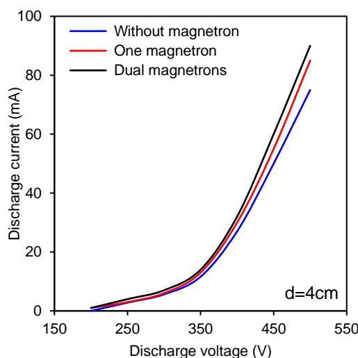
Figure (6) Current-voltage characteristics of discharge plasma at inter-electrode distance of 4cm without magnetron, with only one magnetron and with dual magnetrons
