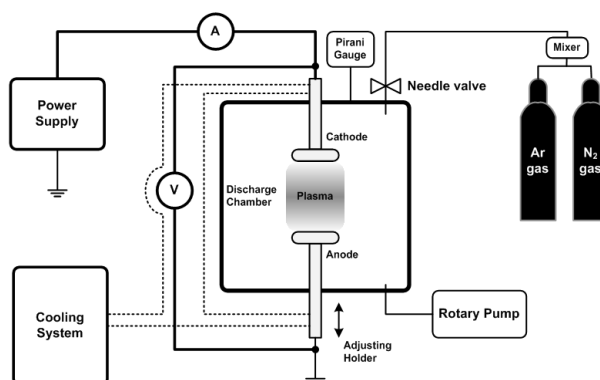
Figure (3) Schematic diagram of the system used in the present work
