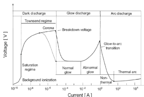
Figure (1) Different regions of plasma discharge on the I-V characteristics [10]
