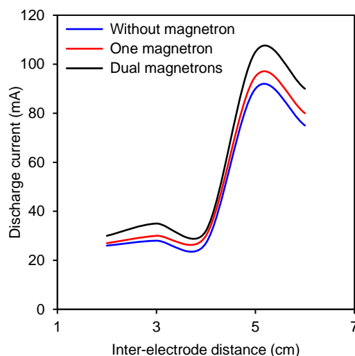
Figure (7) Variation of discharge current with inter-electrode distance at certain discharge voltage (400V) for the cases without magnetron, using one magnetron and dual magnetrons
