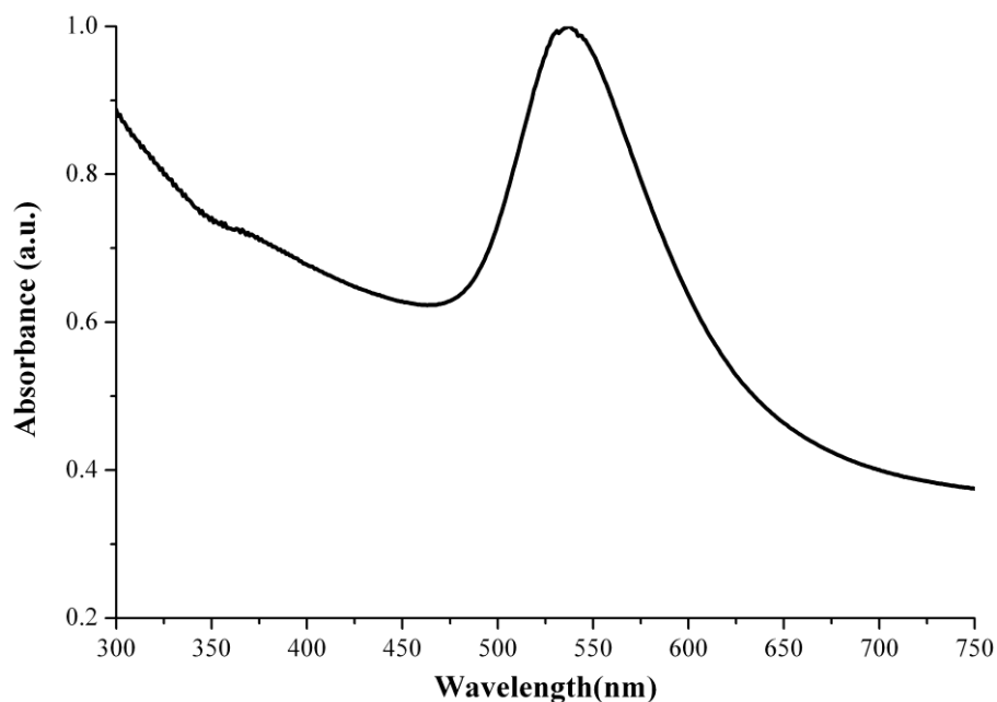
Fig. (2) Absorption spectrum of Au nanoparticles solution
