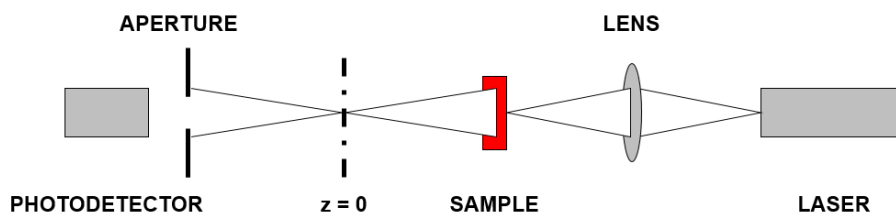
Fig. (1) Schematic illustration of the z-scan setup
