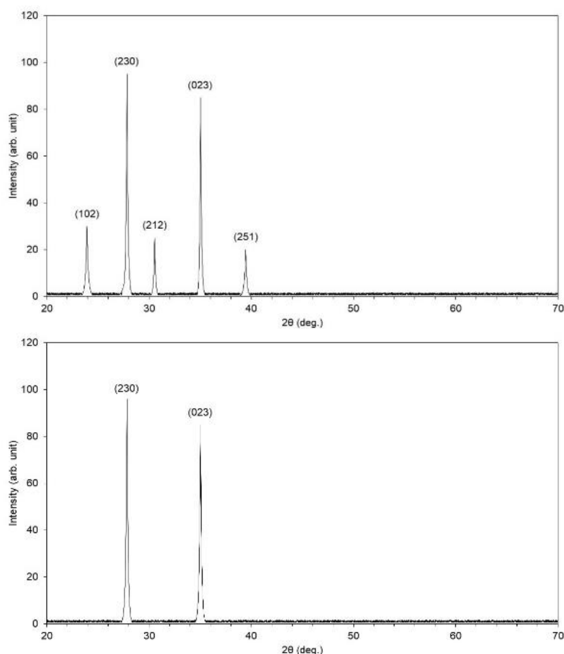
Fig. (2) XRD patterns of the cadmium borate samples prepared in this work using Ar:O 2 mixing ratio of 1:1 and deposition time of 60 s (upper) and 4:1 and 30 s (lower)
