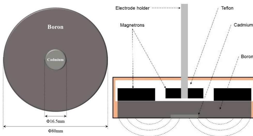
Fig. (1) Configuration of the B and Cd targets and magnetron on the cathode
