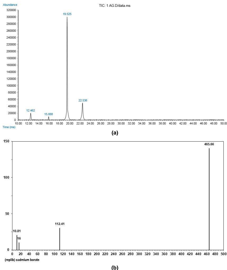
Fig. (5) GC spectrum (a) and MS analysis (b) of the cadmium borate sample prepared using gas mixture of 4:1 and deposition time of 30 s
