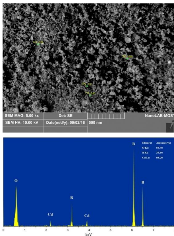
Fig. (4) SEM image and EDS results of the cadmium borate sample prepared using gas mixture of 4:1 and deposition time of 30 s
