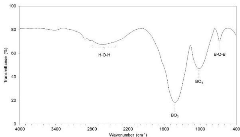
Fig. (3) FTIR spectrum of the cadmium borate samples prepared in this work using Ar:O 2 mixing ratio of 4:1 and deposition time of 30 s
